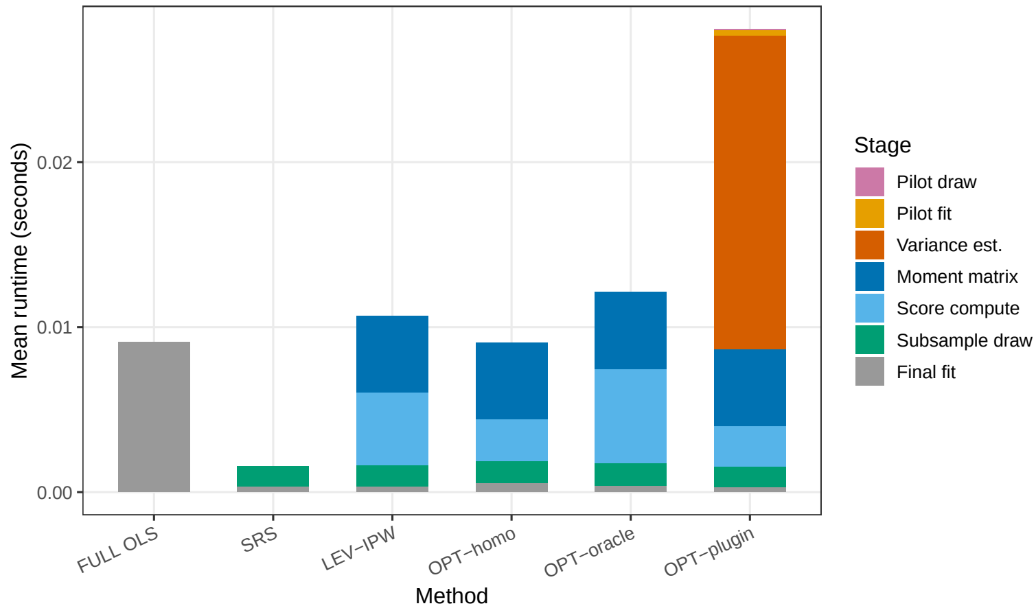
Runtime decomposition by stage (k = 1000, N = 100,000)
